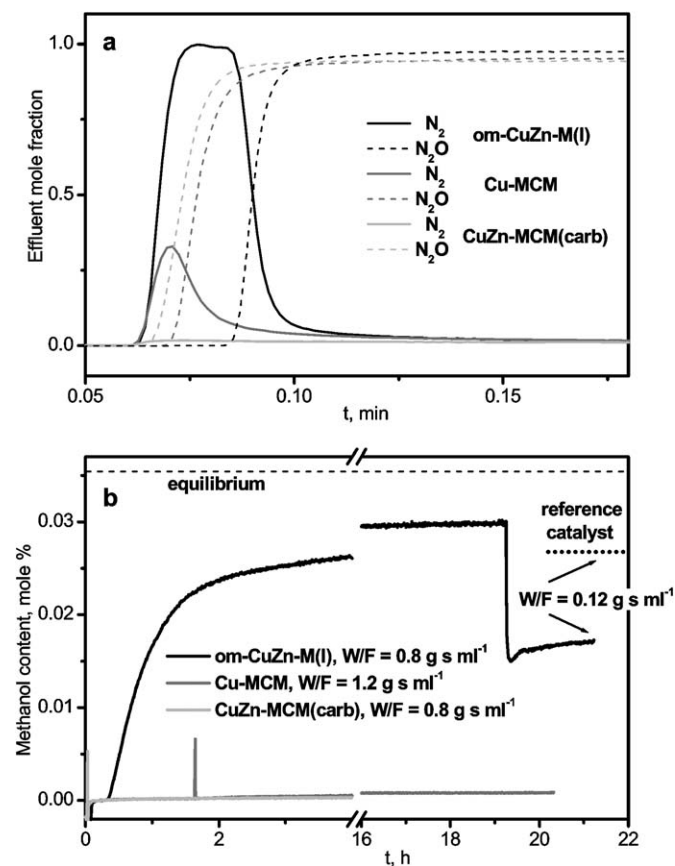
Fig. 5. N_2O frontal chromatography (a) and catalytic behavior in methanol synthesis at normal pressure ((b) T = 493 , K; 72% H_2 , 10% CO , 4% CO_2 and 14% He ) measured with matrix-encapsulated Cu/ZnO catalysts.
